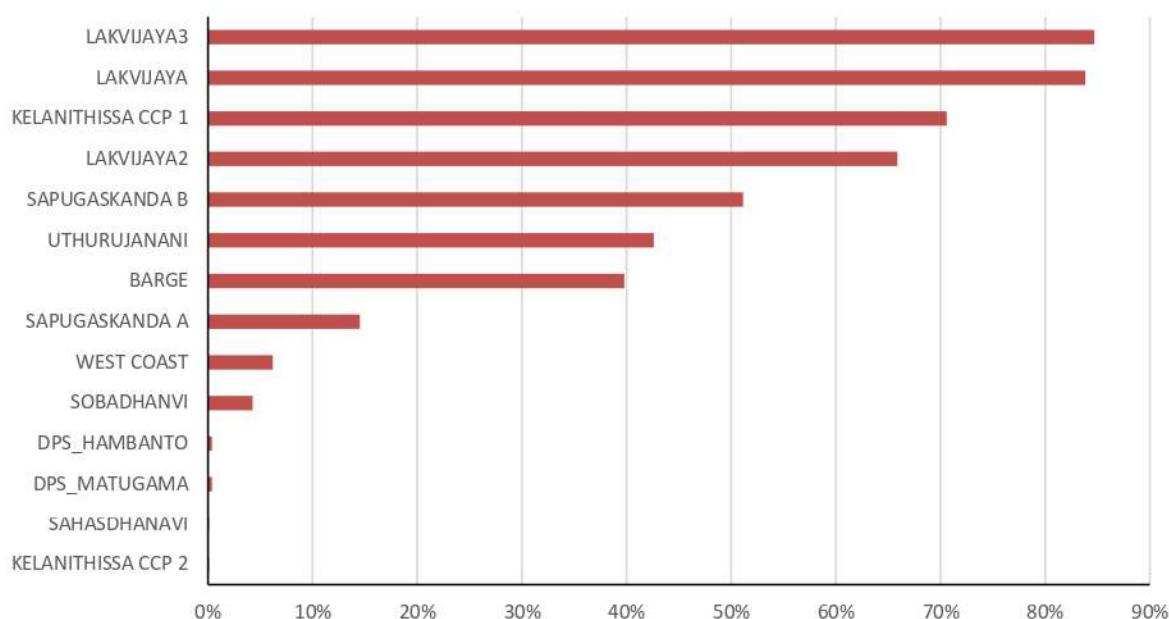
Figure 6 : Plant Factors of Thermal Power Plants in 2028
