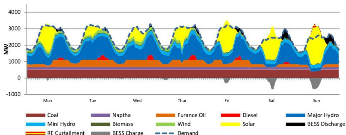
Figure 10: Sample Weekly Dispatch Pattern in 2028 Wet Season (October to December)
