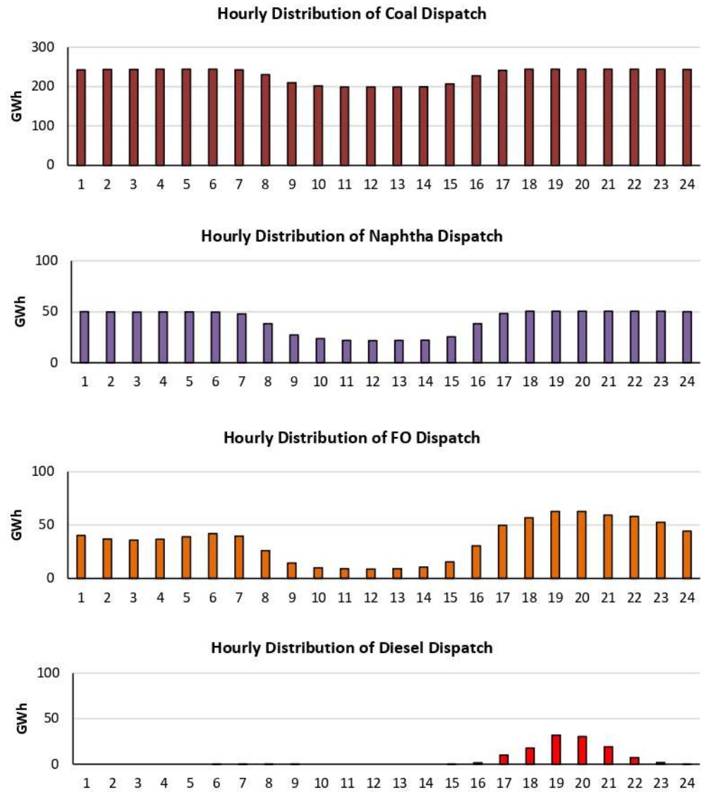
Figure 7: Thermal Power Plant Operation Pattern in 2028
