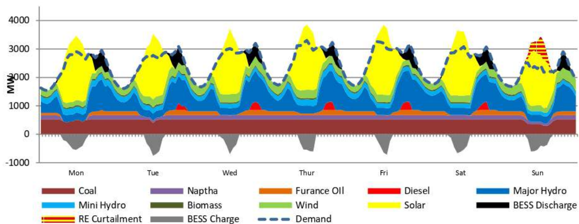
Figure 9: Sample Weekly Dispatch Pattern in 2028 High Wind Season (May to September)
