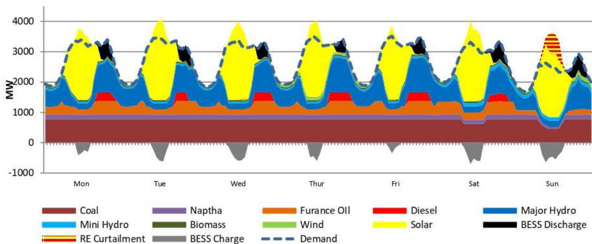
Figure 8: Sample Weekly Dispatch Pattern in 2028 Dry Season (January to April)
