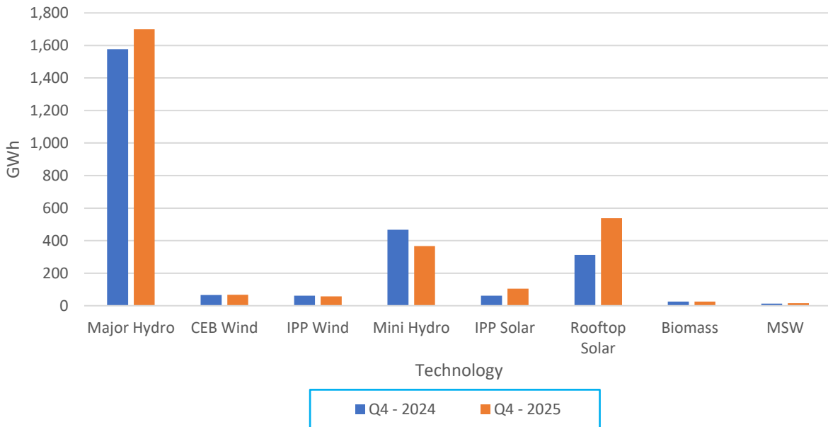
Comparison of RE Generation between Q4 2024 and Q4 2025
