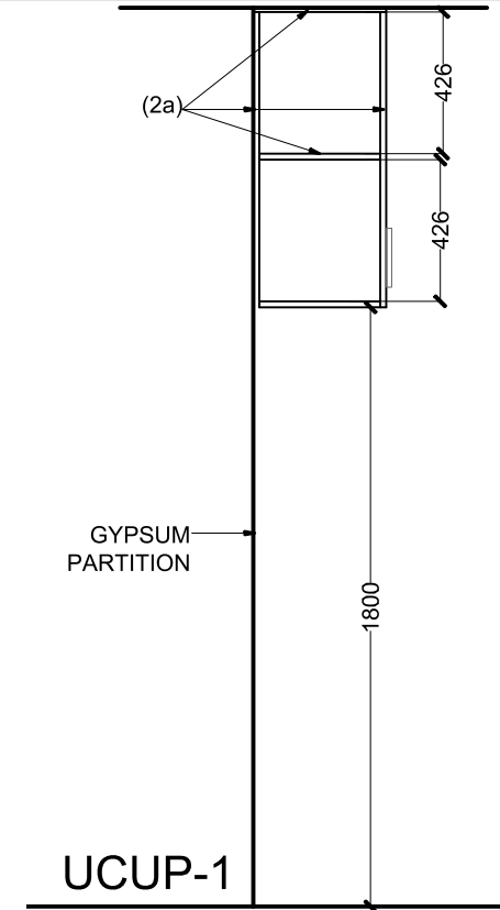
SECTION-X-X
