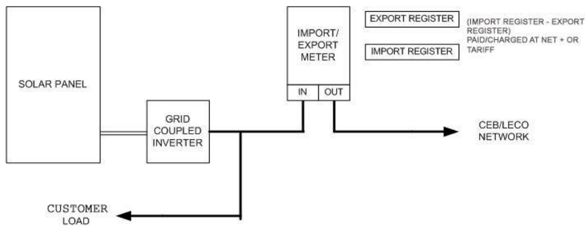
SCHEME 2 NET ACCOUNTING
