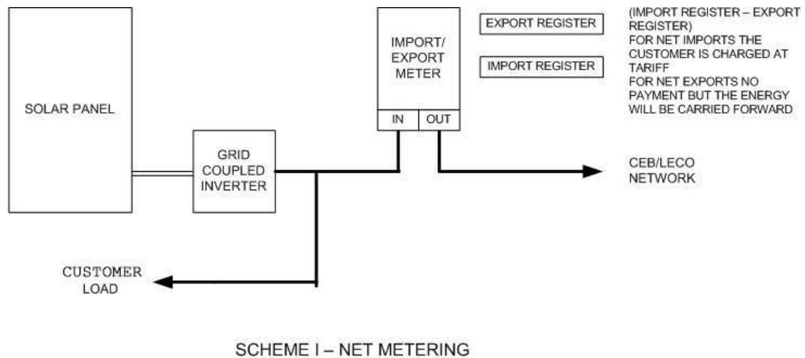
Figure 1: Typical connection arrangement for the Scheme 1 is given in the Annexure 01.
