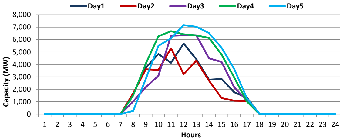
A5.17 Modelled Plant output variation of 10MW at kilinochchi area for consecutive 5 days
