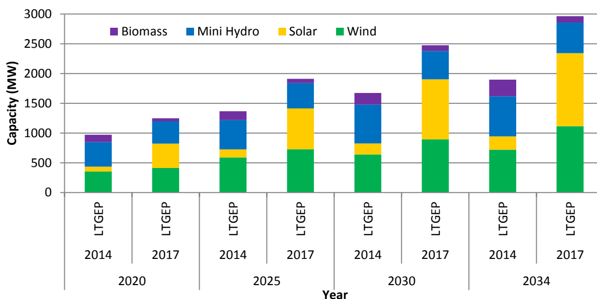
Figure 10.4 – Comparison of ORE Capacity Addition between LTGEP 2017 & LTGEP 2014
