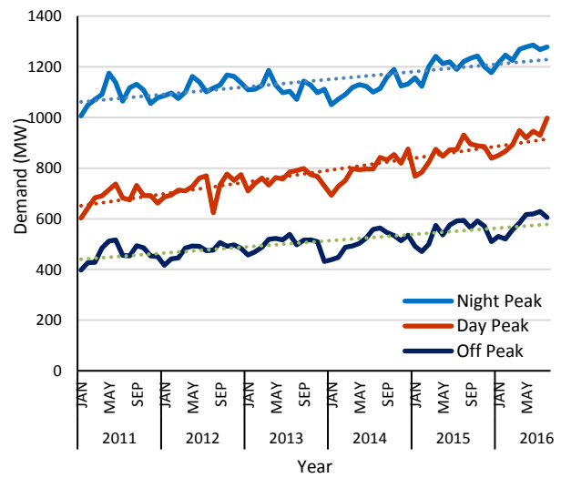
Figure 10.1(b) - Demand variation of Whole Country without Western Province
