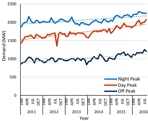
Figure 10.1(a) - Demand variation of Whole Country
