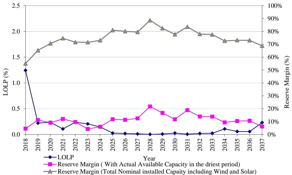
Figure 7.11 – Variation of Critical Reserve Margin and LOLP in Base Case
