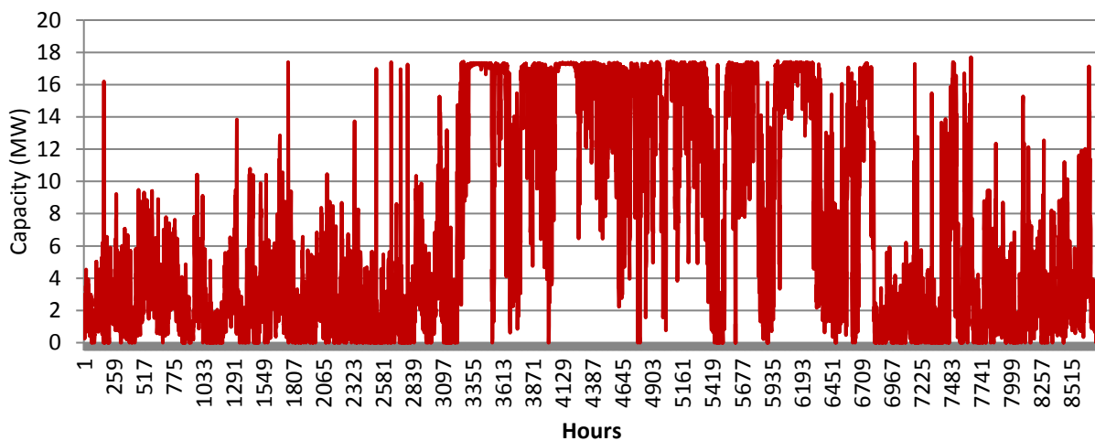
Fig. A5.9: Wind Plant Power output
