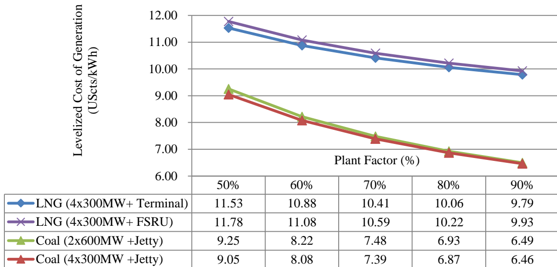
Figure 7.15: Screening Curves for LNG and Coal Power Plants of 1200MW
