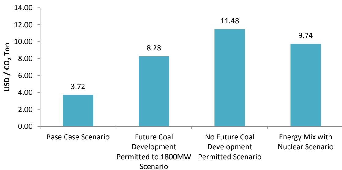
Figure 9.12 – Comparison of Incremental Cost for CO 2 reduction
