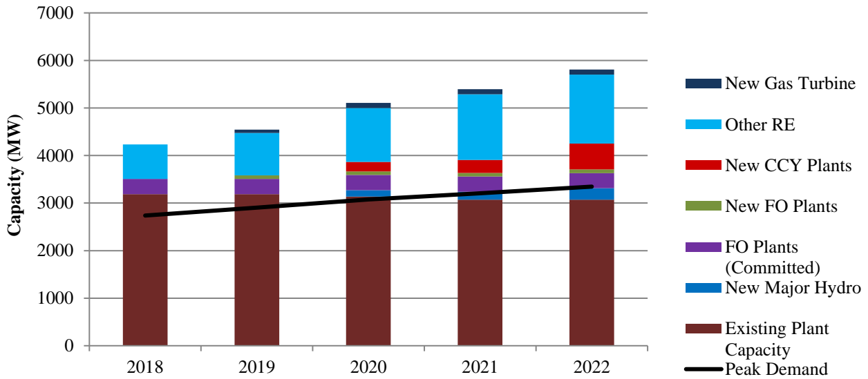
Figure 11.2 – Installed Capacity with Peak Demand (Contingency Event 1)
