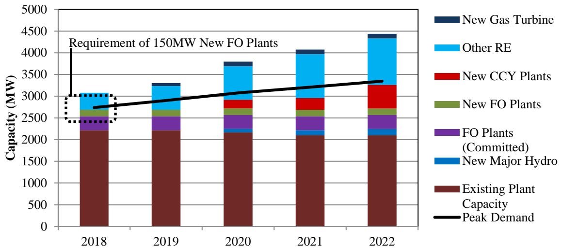
Figure 11.4 - Available Capacity in Critical Period with Peak Demand (Contingency Event 2)
