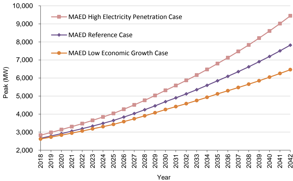
Figure 3.9 – Peak Demand Forecast Comparison
