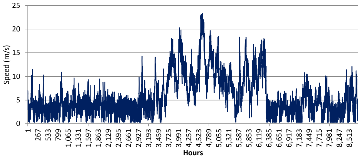
Fig. A5.14: Wind speed variation
