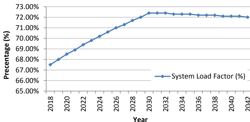
Figure 3.7 – System Load Factor Forecast 2018-2042
