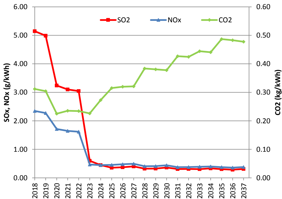
Figure 9.5 – SO 2 , NO x and CO 2 emissions per kWh generated
