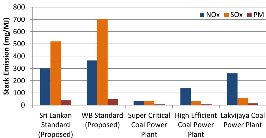
Figure 9.3 - Comparison of Stack Emission Standards and Stack Emission Levels of Coal Power Plants
