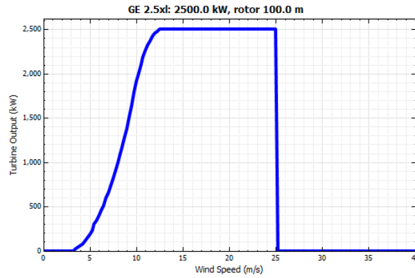
Fig. A5.1: Power curve of the modelled wind turbine
