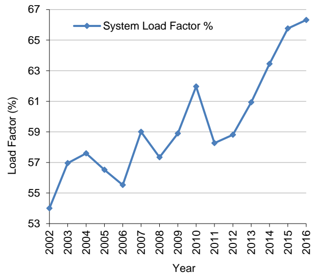
Figure 3.2 – Past Trend in the Load Factor
