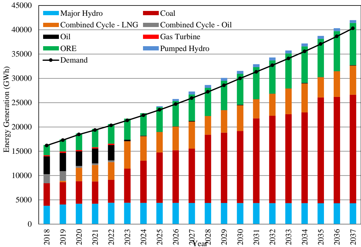
Figure 7.4– Energy Mix over next 20 years in Base Case
