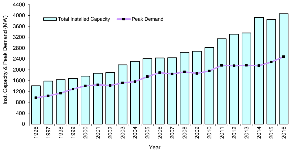
Figure 1.10 – Total Installed Capacity and Peak Demand
