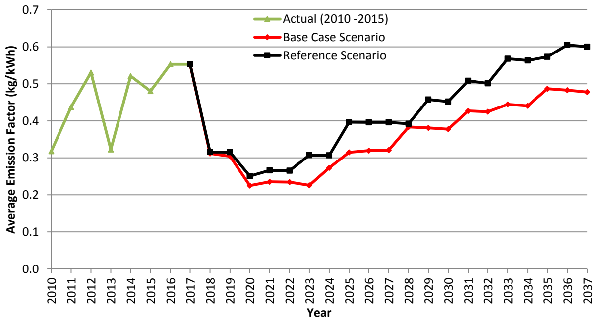
Figure 9.10 – Average Emission Factor Comparison
