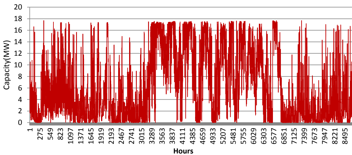
Fig. A5.6: Wind Plant Power output
