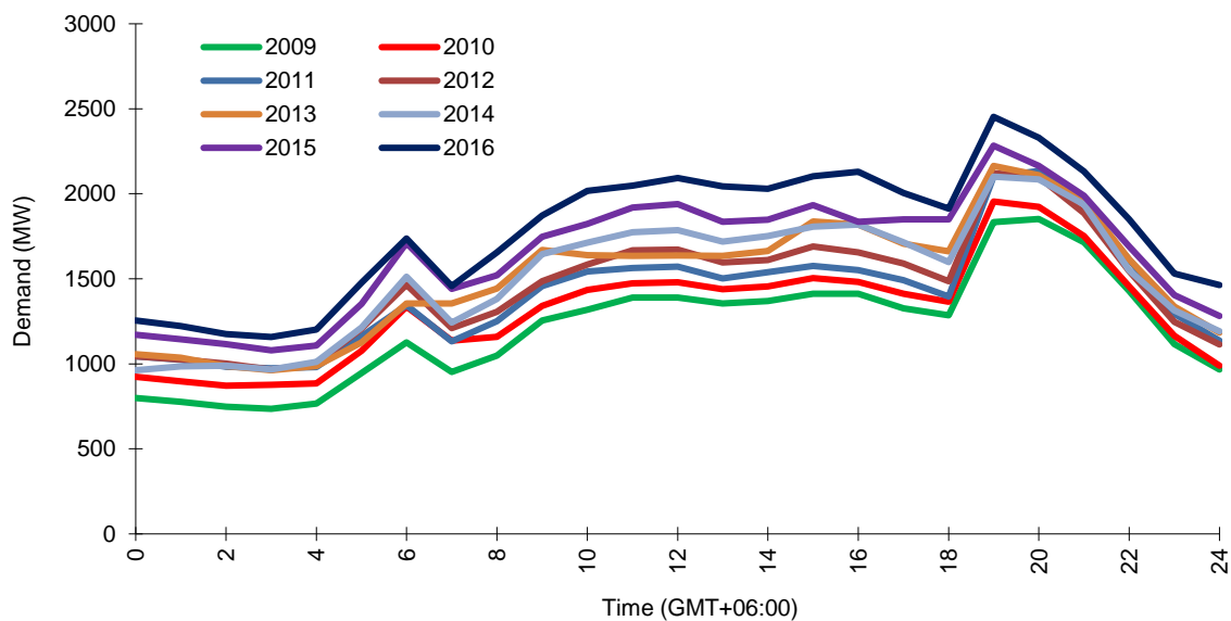
Figure 3.3 - Change in Daily Load Curve Over the Years
