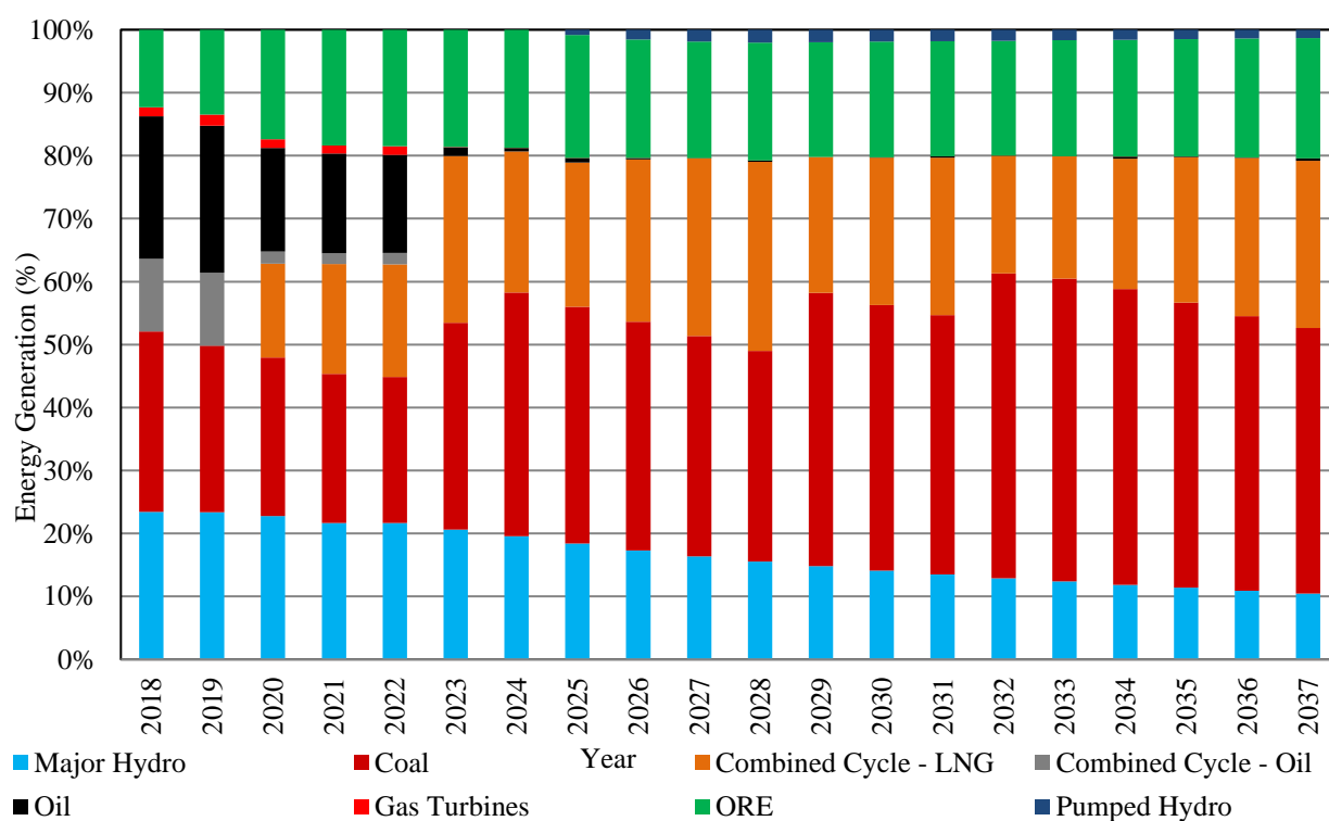
Figure 7.13 –Percentage Energy Contribution by Plant Type of Future Coal Development Limited to 1800MW Case
