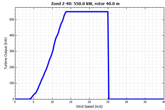
Figure A5.13: Power curve of the modelled wind turbine
