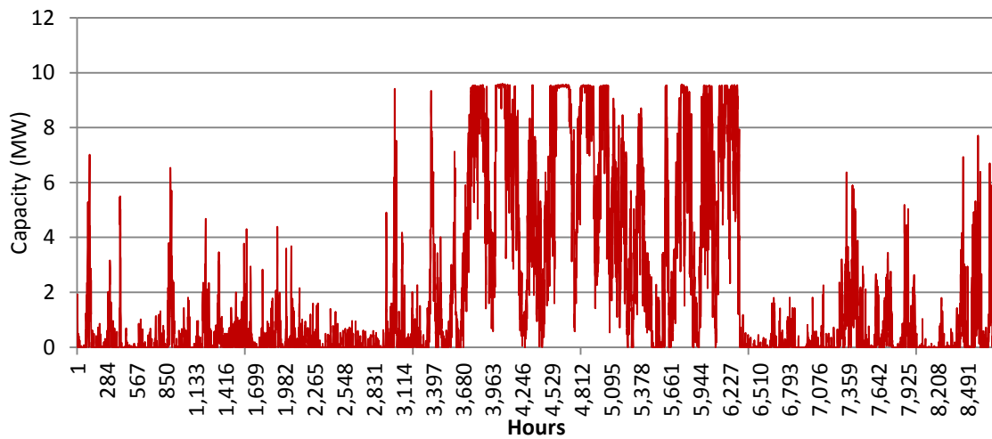
Fig. A5.15: Wind Plant Power output
