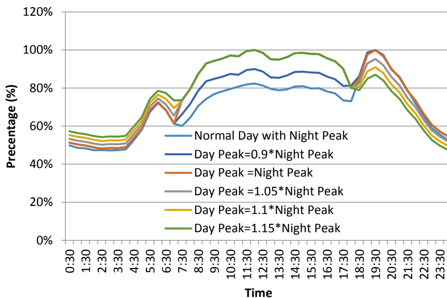
Figure 3.6 – Load Profile Shape Forecast
