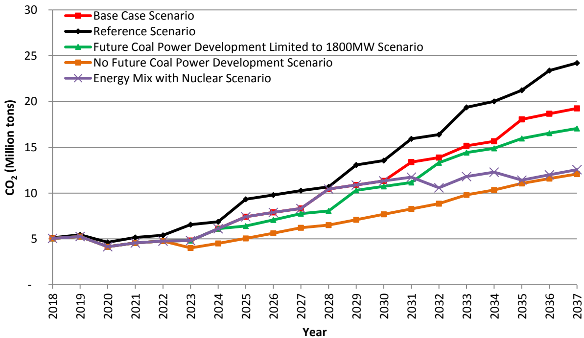
Figure 9.8 – CO 2 Emissions
