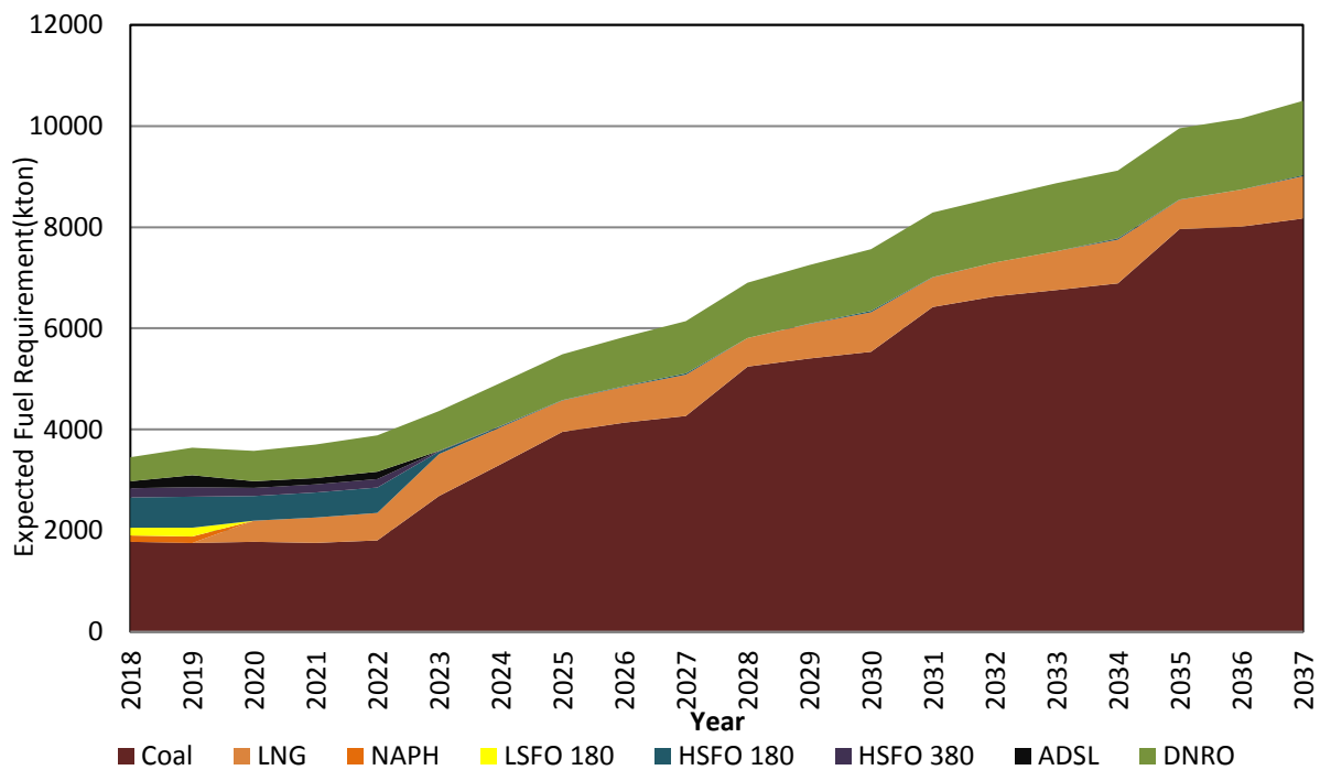
Figure 7.8- Fuel Requirement of Base Case
