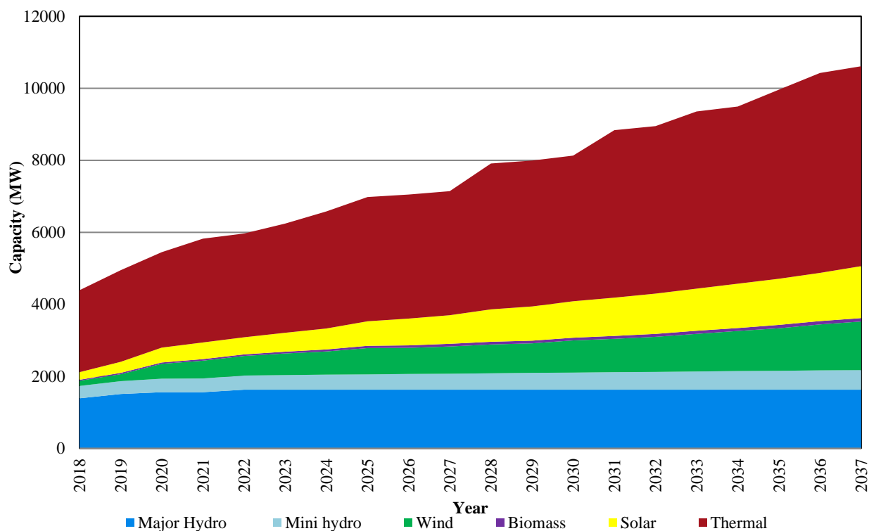
Figure 7.3 – Capacity wise Renewable Contribution over next 20 years
