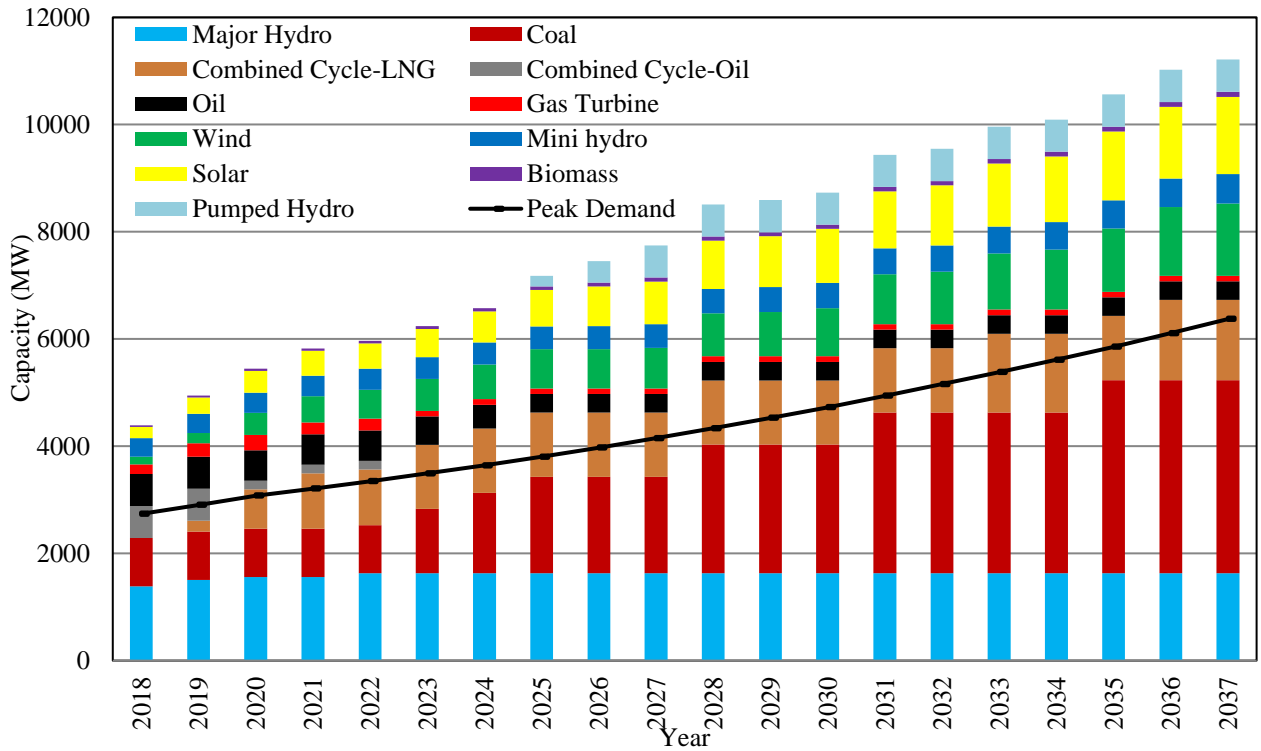
Figure 7.1 – Cumulative Capacity by Plant Type in Base Case
