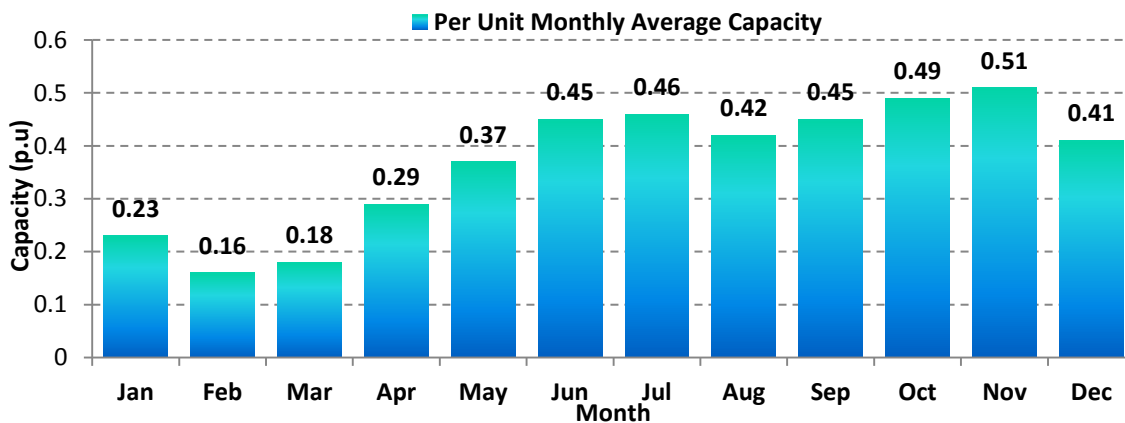
A5.18 Per unit Monthly average capacity of Mini Hydro plant model
