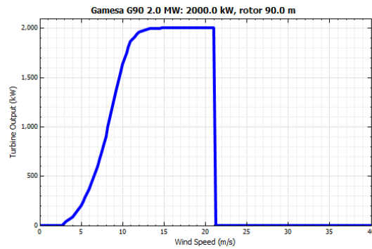
Fig. A5.10: Power curve of the modelled wind turbine
