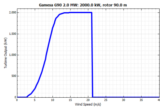
Fig. A5.7: Power curve of the modelled wind turbine
