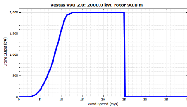
Fig. A5.4: Power curve of the modelled wind turbine
