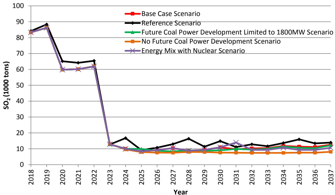
Figure 9.6 – SO 2 Emissions
