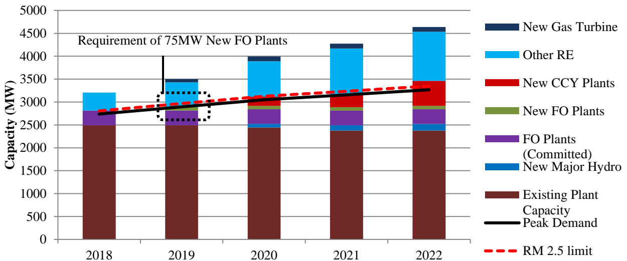
Figure 11.3 - Available Capacity in Critical Period with Peak Demand (Contingency Event 1)
