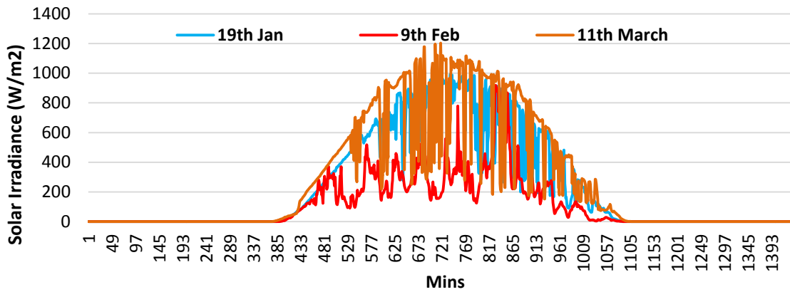
A5.16 Actual Measured Solar Irradiance variation for 3 days in 2015 (1 minute resolution)
