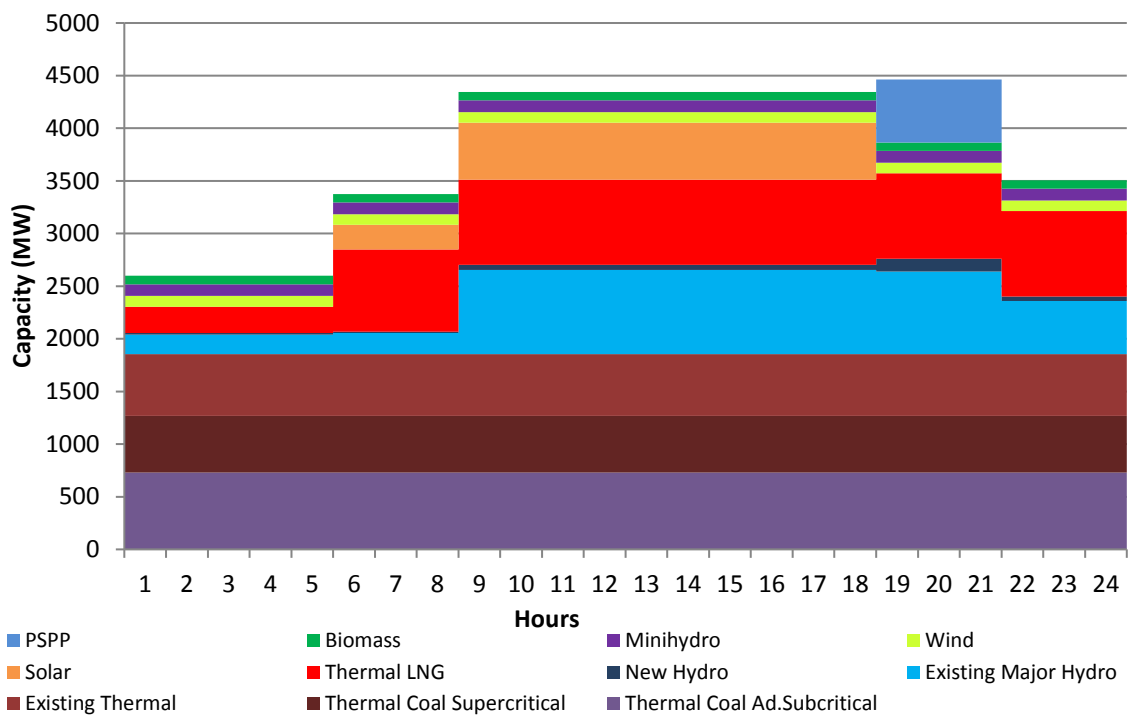
Figure 7.12 – Capacity Contribution from Power Plant in a Day in March /April 2028
