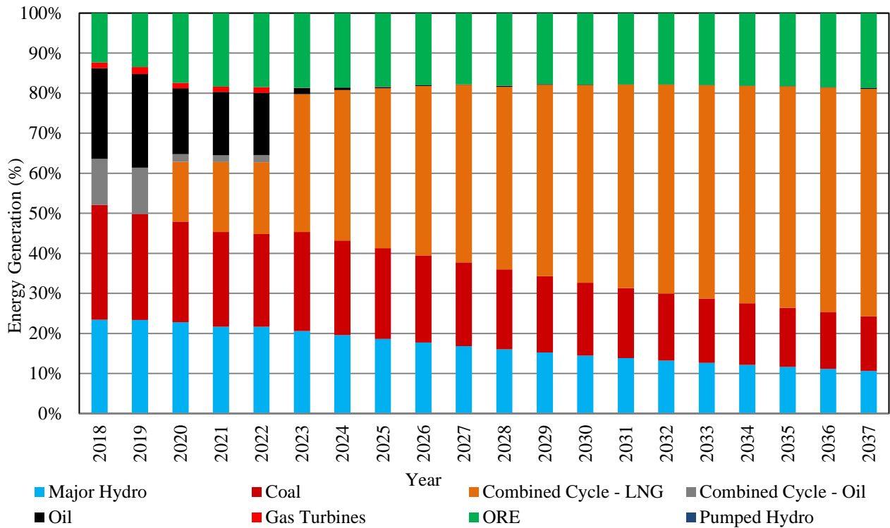
Figure 7.14 –Percentage Energy Contribution by Plant Type of No Future Coal Power Development Case
