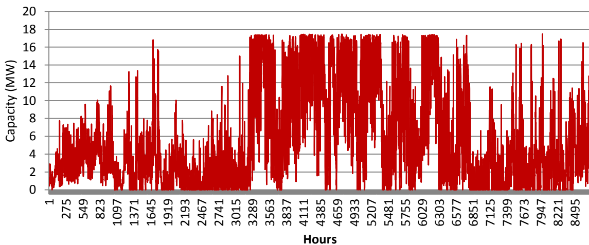
Fig. A5.12: Wind Plant Power output
