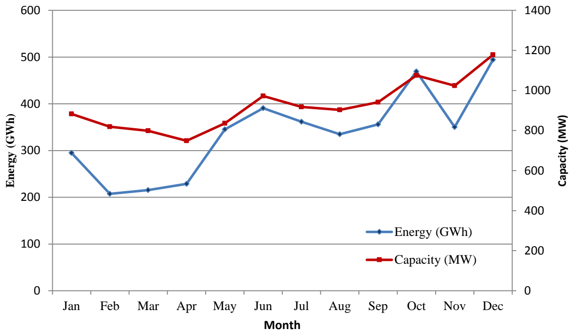
Figure 2.3 - Monthly Average Hydro Energy and Capacity Variation
