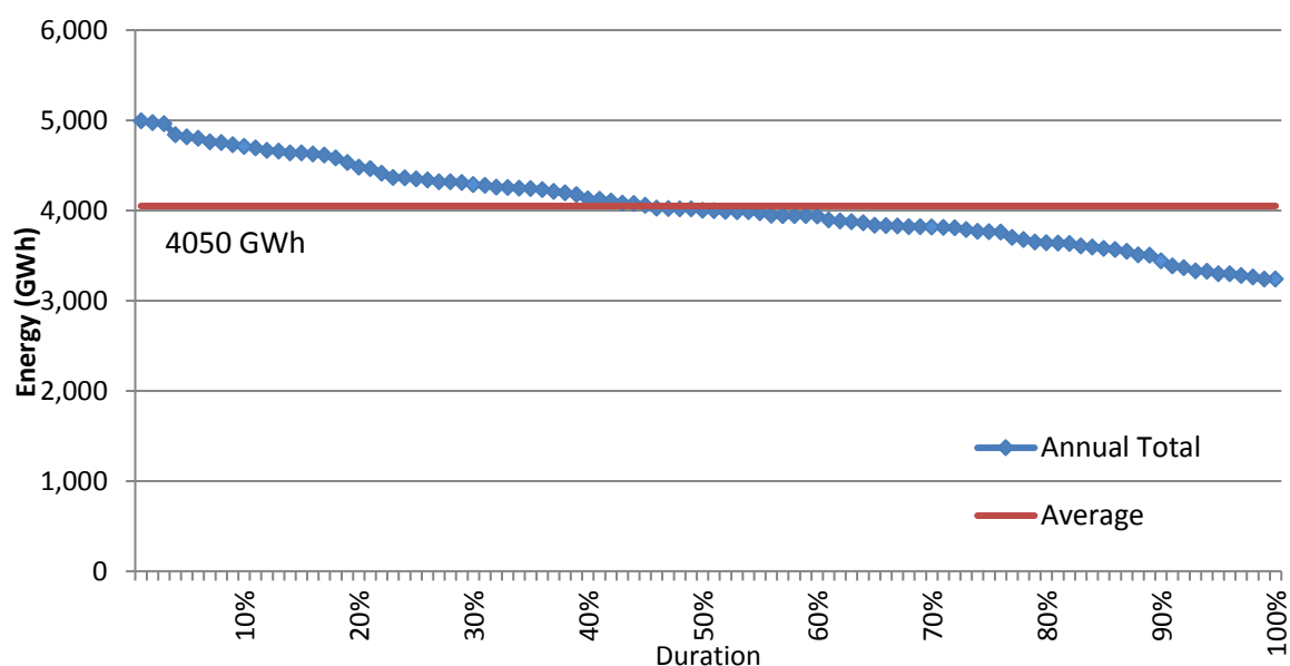
Figure 2.2 - Potential of Hydropower System from Past 35 years Hydrological Data
