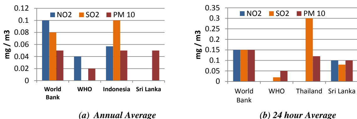
Figure 9.2 - Comparison of Ambient Air Quality Standards
