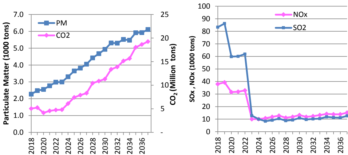
Figure 9.4 – PM, SO 2 , NO x and CO 2 emissions of Base Scenario
