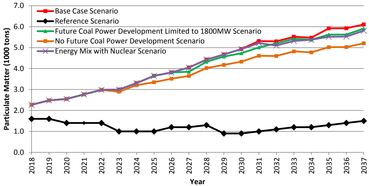
Figure 9.9 – Particulate Matter Emissions
