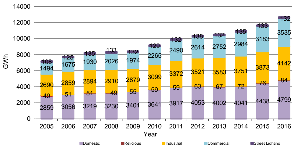
Figure 1.6 - Sectorial Consumption of Electricity (2005 - 2016)
