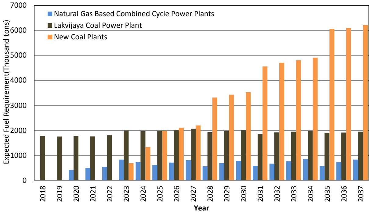
Figure 7.10- Expected Annual Coal and Natural Gas Requirement of the Base Case
