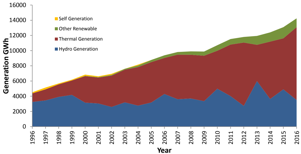
Figure 1.12 - Hydro Thermal Share in the Recent Past
