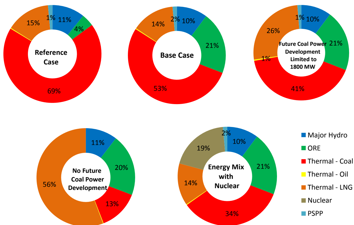
Figure 7.16: Energy share comparison in 2037
