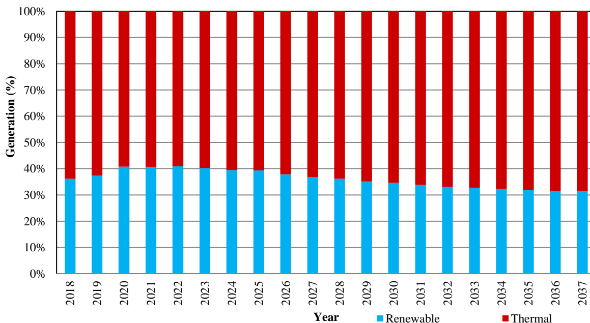
Figure 7.7 Percentage Share of Renewables over next 20 years in Base Case
