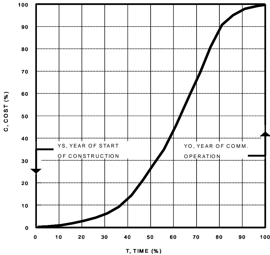
Plant capital cost distribution against time
