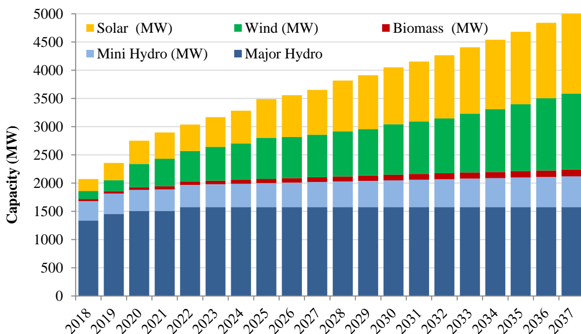
Figure 5.2: Renewable Energy Capacity Development
