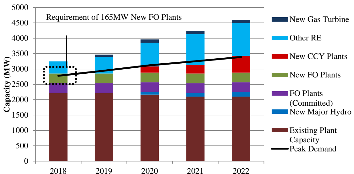
Figure 11.5 - Available Capacity in Critical Period with Peak Demand (Contingency Event 3)
