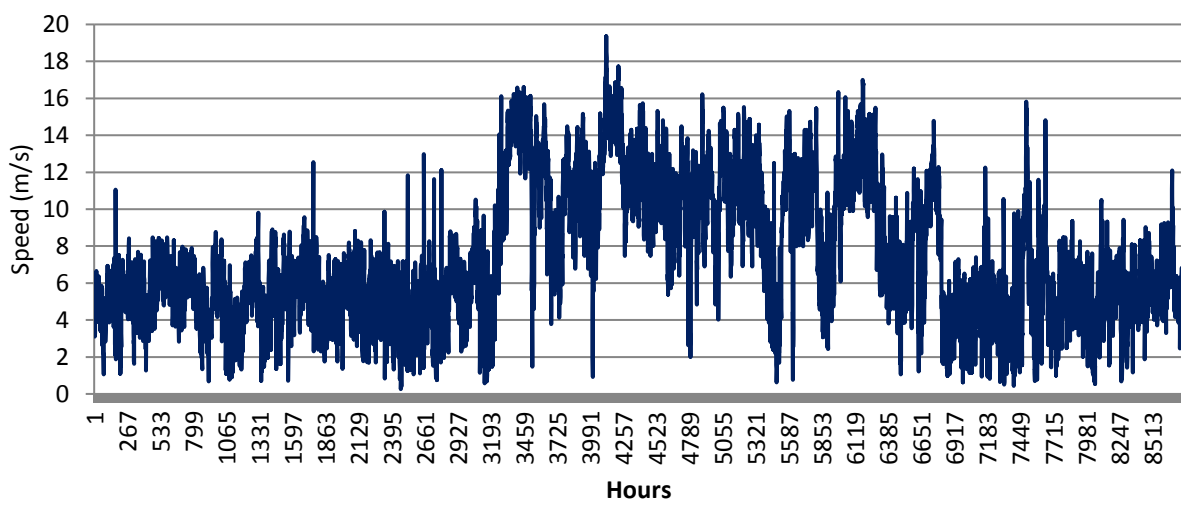
Fig. A5.8: Wind speed variation
