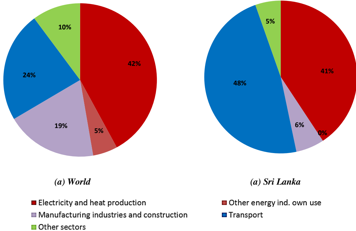
Figure 1.4 - CO 2 Emissions from Fuel Combustion 2014
