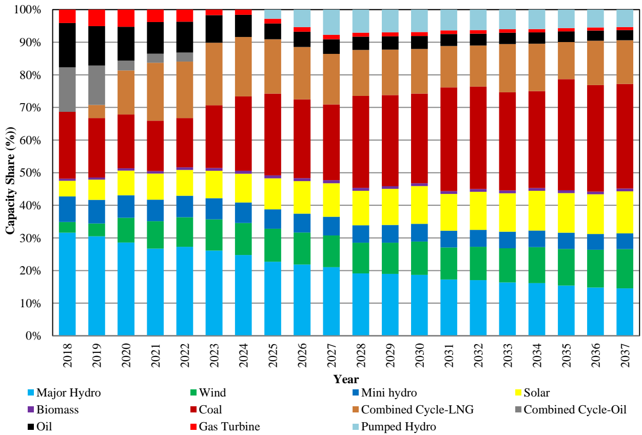
Figure 7.2 – Capacity Mix over next 20 years in Base Case
