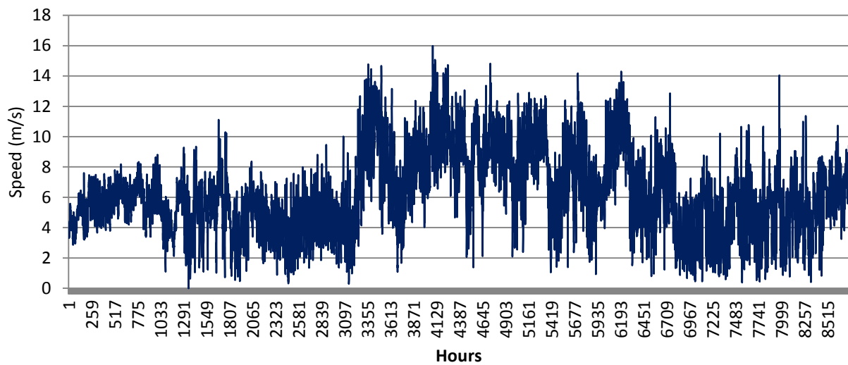
Fig. A5.11: Wind speed variation
