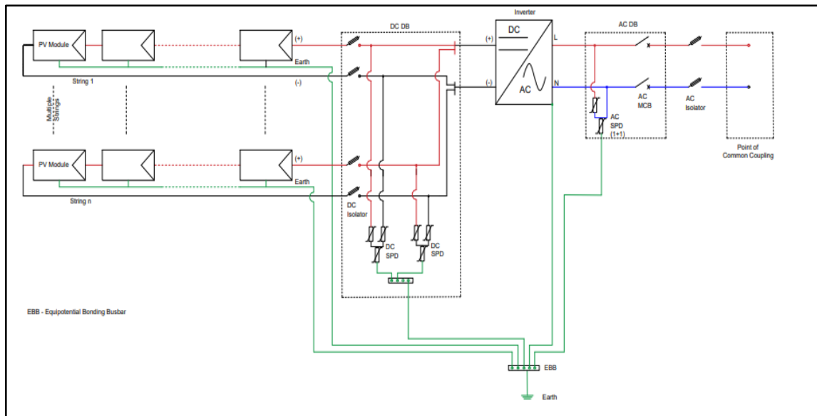
Figure 3-9: Connection diagram for Single Phase-Multi String
