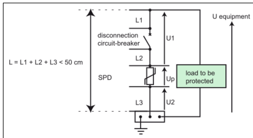
Figure 3 6: Connections of a SPD L < 50 cm
