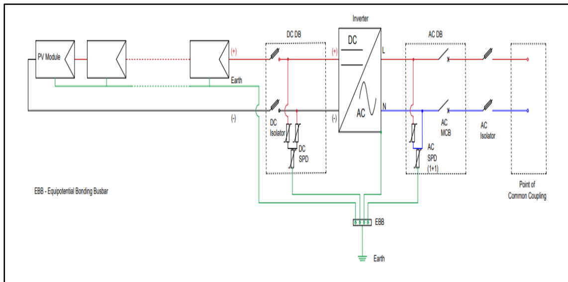
Figure 3-8: Connection diagram for Single Phase-Single String
