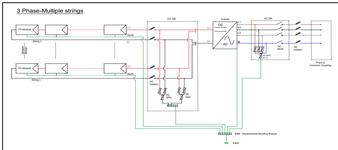
Figure 3-10: Connection diagram for Three Phase-Multi String
